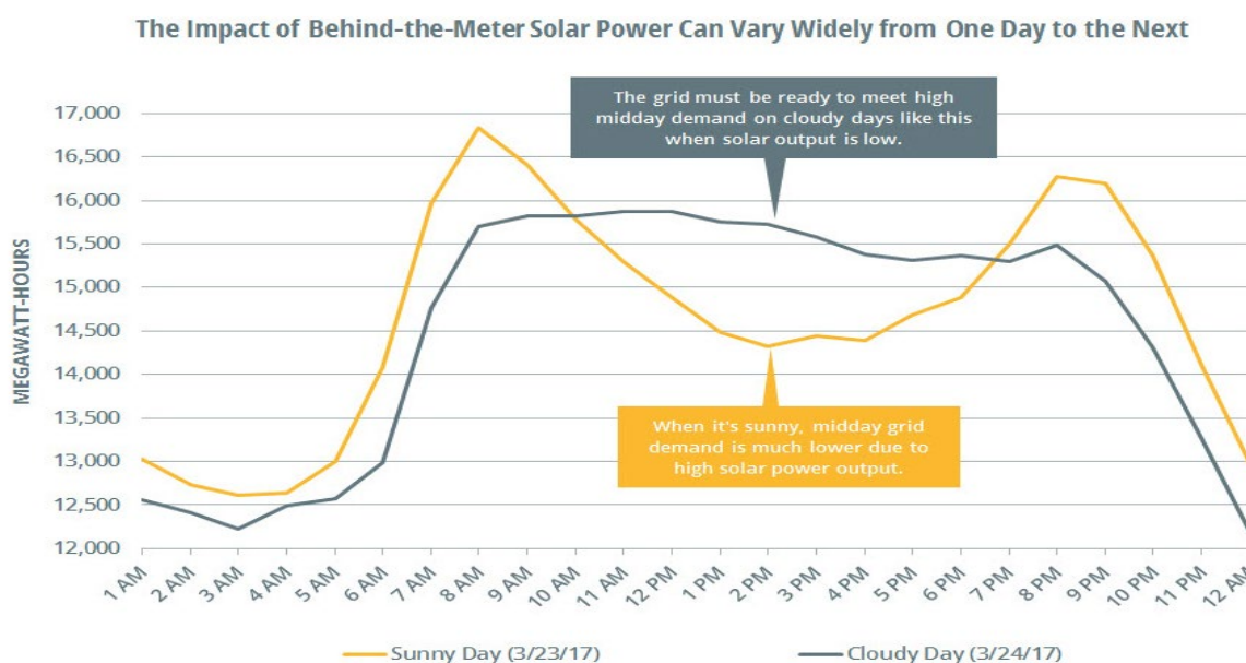
Figure 51: ISO-NE load shape with and without solar 173
