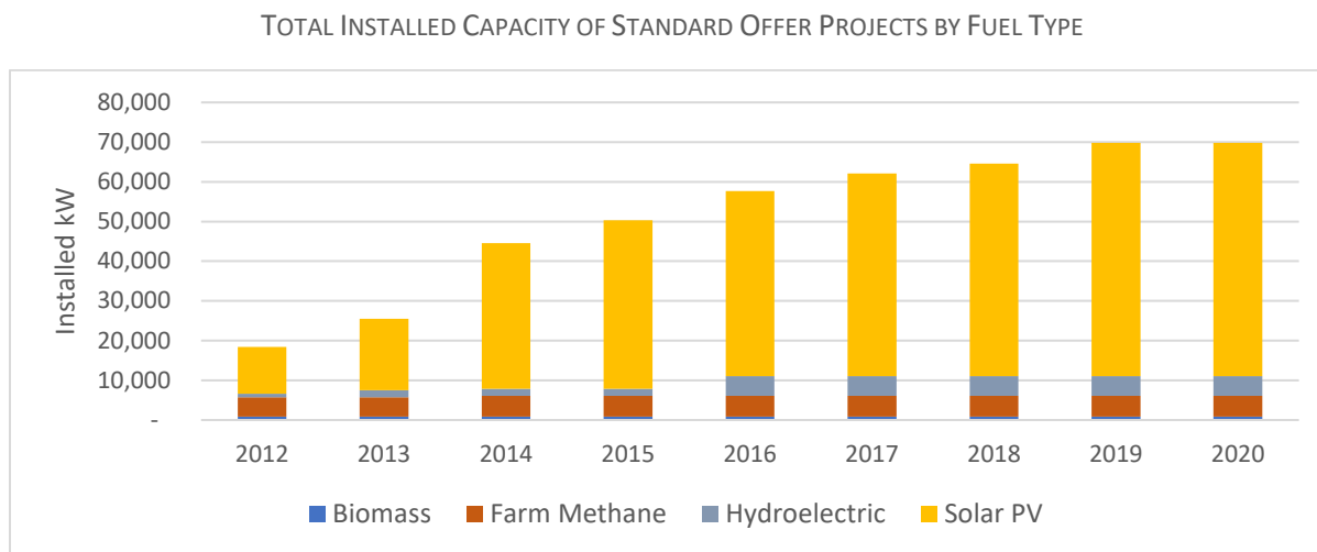
Figure 32: Installed capacity of Standard Offer projects by fuel type
