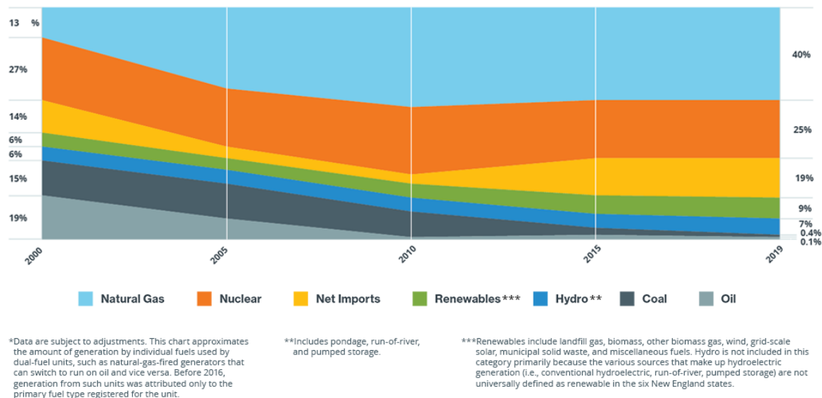
Figure 37: ISO-NE Electric Energy Generation
