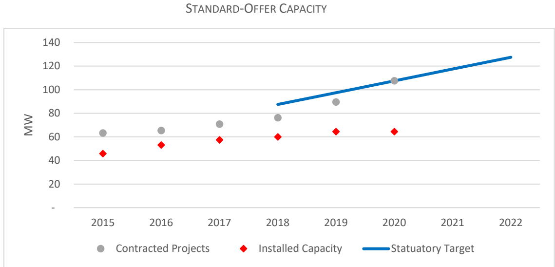
Figure 31: Actual historical installed capacity, contracted capacity, and cumulative contracted capacity targets through 2022.
